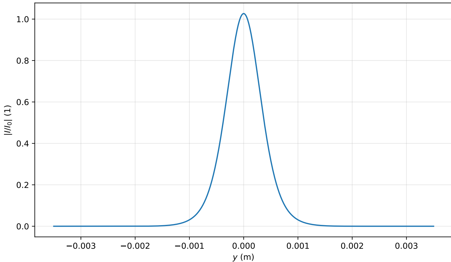
Intensity profile I(x=0, y, z=1.672)/I_0 , P_{in}=0.6P_{cr} , artificial time
